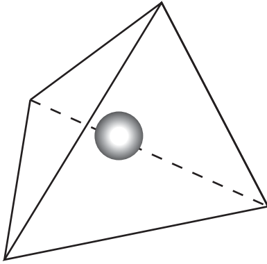
A tetrahedron with a hole.
