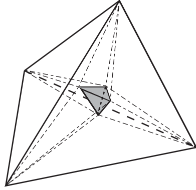
A subdivision of the tetrahedron.
